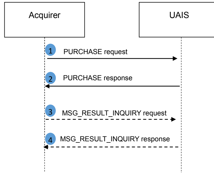
Figure 2: Flow of Consumer-presented QRC-based Purchase
