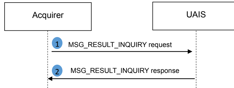
Figure 9: Flow of Message Result Inquiry
