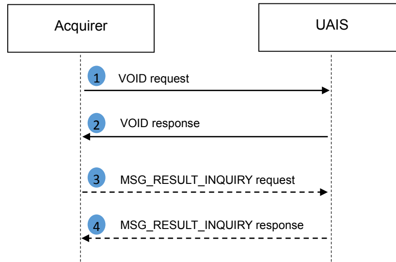
Figure 7: Flow of Purchase Cancellation
